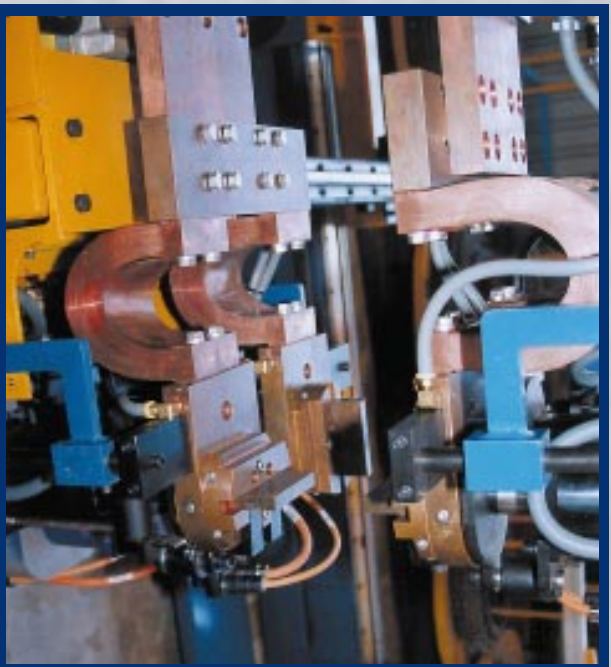
360° Rotating and/or Raise and Lower Heads
